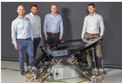
MB-E-6DOF/12/1500KG Gen3 shown with optional moving plate frame
