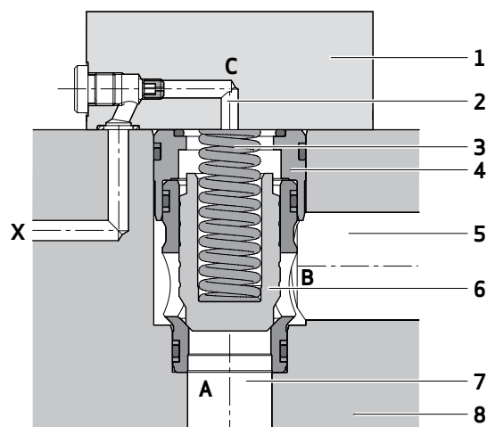
Directional Cartridge Valve and Cover
